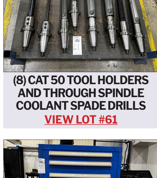
(8) CAT 50 TOOL HOLDERS AND THROUGH SPINDLE COOLANT SPADE DRILLS
