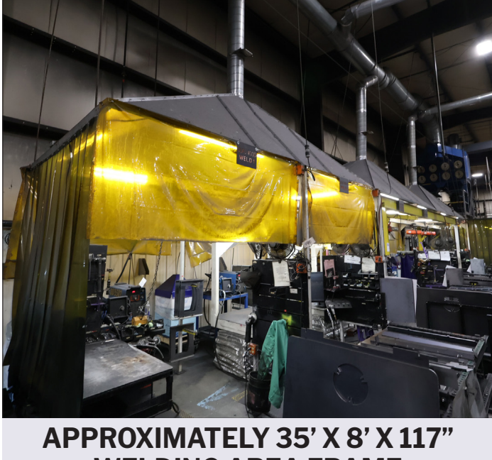
APPROXIMATELY 35' X 8' X 117" WELDING AREA FRAME VIEW LOT #40
