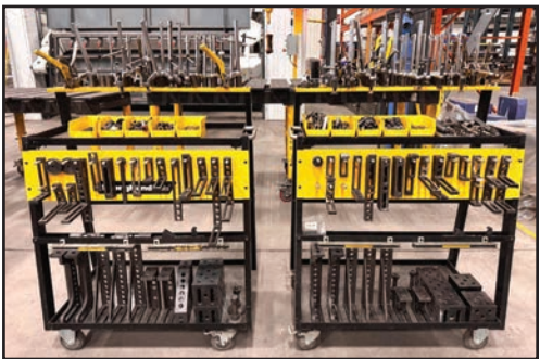
BUILDPRO FIXTURE COMPONENTS
