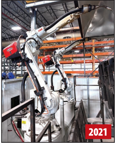
ABB TWIN ROBOT MIG WELDING CELL
