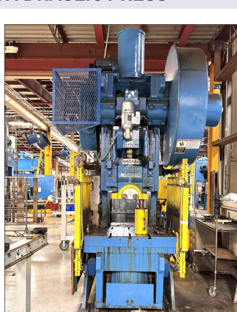
NIAGARA A110-GRD OBI GEARED PUNCH PRESS
