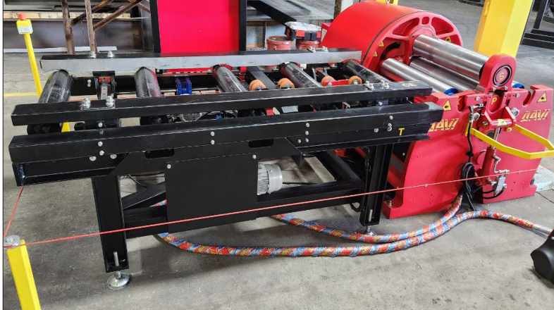
DAVI MCA 0615 5/16" X 24" 4-ROLL HYDRAULIC PLATE ROLL
