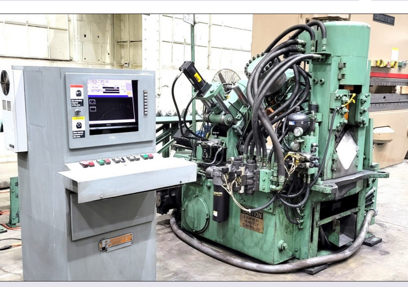
PEDDINGHAUS AFPS 623L 6" X 6" X 1/2" CNC ANGLEMASTER PUNCH & SHEAR LINE
