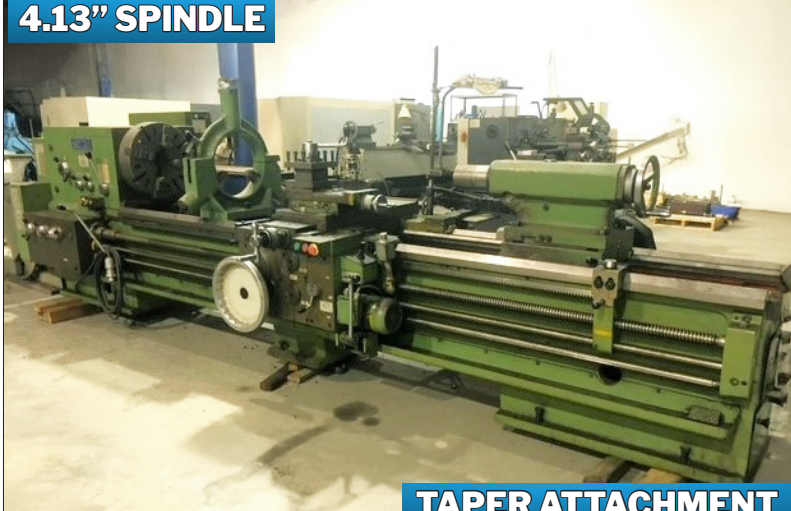
4.13" SPINDLE TAPER ATTACHMENT 27.5" X 118" RYAZAN 1M63H GAP BED LATHE VIEW LOT #132
