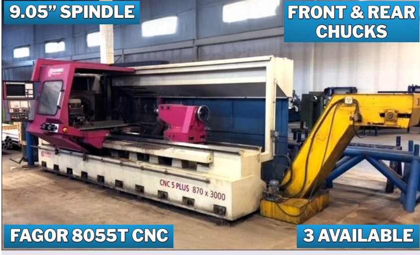
9.05" SPINDLE FRONT & REAR CHUCKS FAGOR 8055T CNC 34" X 118" GEMINIS CNC 5 PLUS 870 X 3000 CNC HOLLOW SPINDLE LATHE VIEW LOTS #101, 102 & 103
