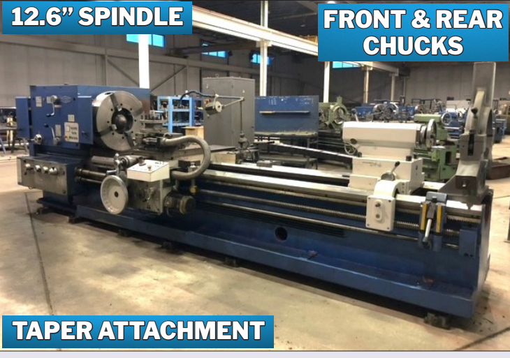
12.6" SPINDLE FRONT & REAR CHUCKS TAPER ATTACHMENT 31" X 122" RYAZAN RT-983-3 HOLLOW SPINDLE LATHE VIEW LOT #91
