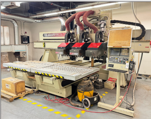
KOMO MACH III VR-1005TT 3-SPINDLE CNC ROUTER
