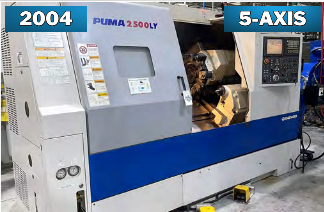
DAEWOO PUMA 2500LY 5-AXIS CNC TURNING CENTER
