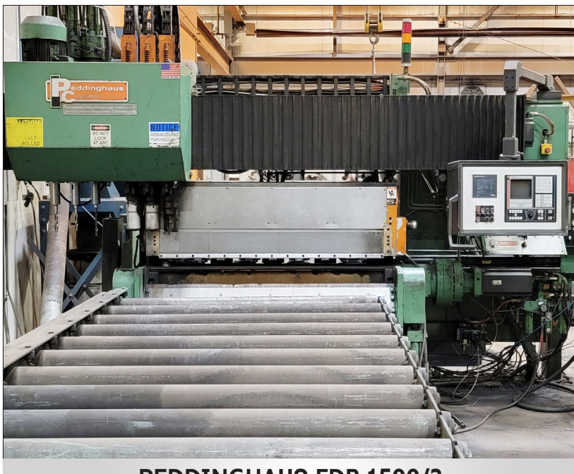
PEDDINGHAUS FDB 1500/3 PLATE PROCESSING SYSTEM
