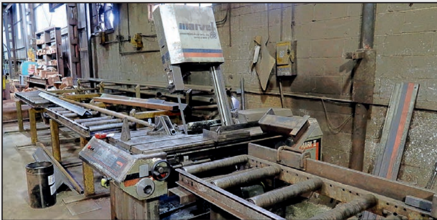
Marvel Series 8-Mark-II Vertical Tilt-Frame Band Saw
