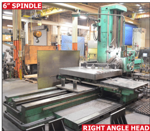
VWF BFN 125 table-type horizontal boring mill
