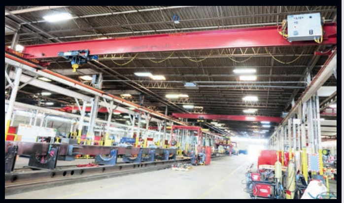
(2) 4-Ton x 48' Span Radio Control Bridge Cranes and Crane Rail
