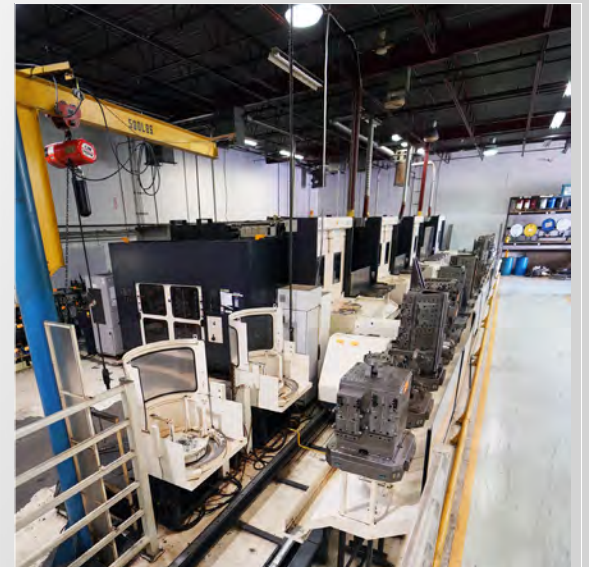
MAKINO A88/A88E LINE, 4 CNC HORIZONTAL MACHINING CENTERS WITH 32 PALLET SHUTTLE SYSTEM
