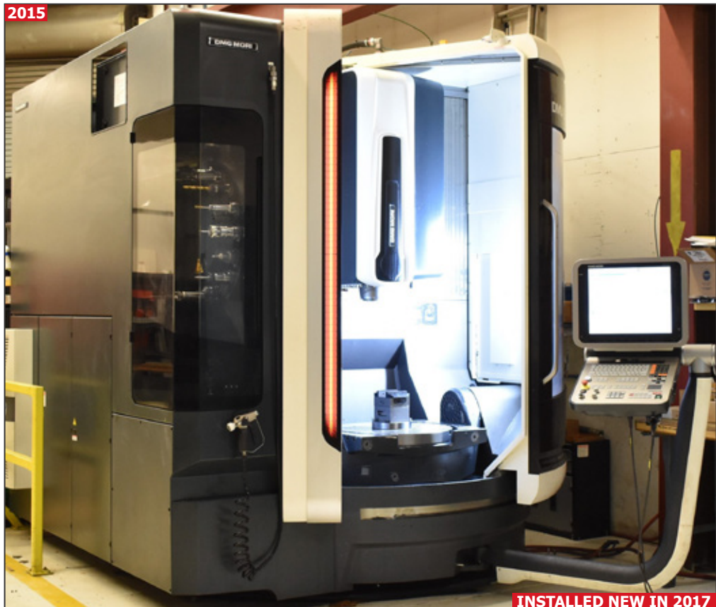
DMG MORI MU65 MONOBLOCK, 5-Axis CNC vertical machining center
