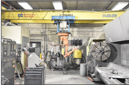
TAFa-THERMAC robotic metalizing spray weld cell with ABB (2005) IRB2400 6-axis gun welding robot
