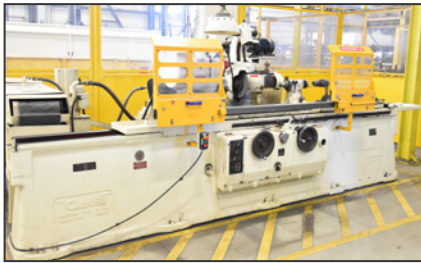
CHURCHILL PBW universal cylindrical grinder
