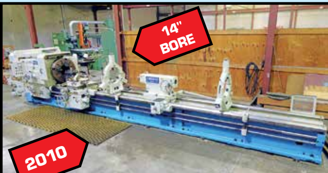
SPARK 39" X 20' HOLLOW SPINDLE LATHE
