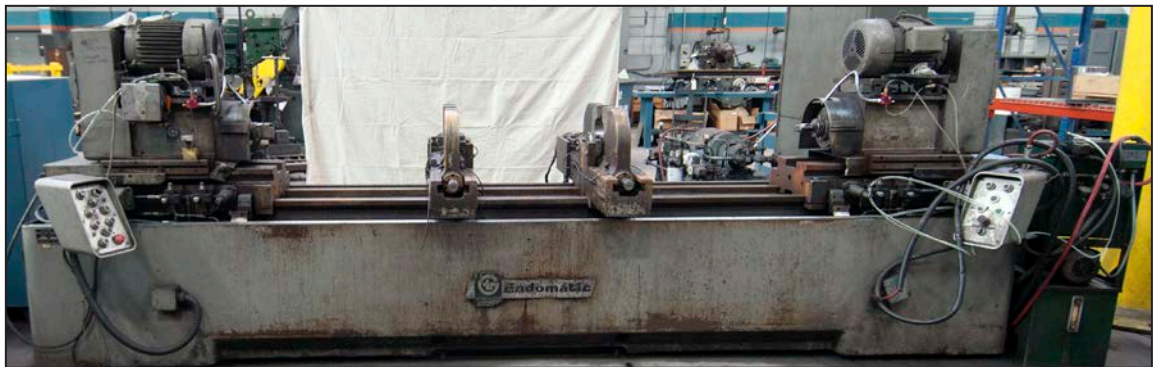
GIDDINGS & LEWIS ENDOMATIC HDB facing and centering machine
