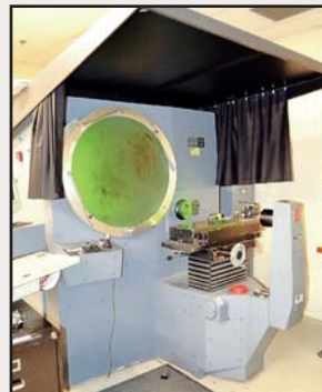
30" Jones & Lamson "Epic 30E" Optical Comparator
