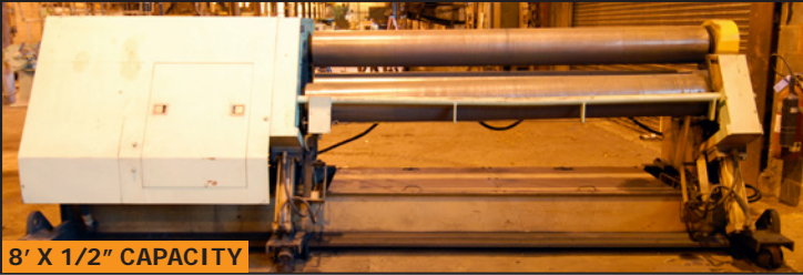
BERTSCH initial type hydraulic pinch bending rolls
