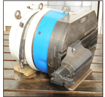
D'ANDREA CNC facing head
