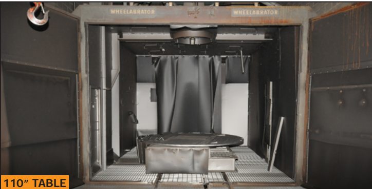
WHEELABRATOR rotary table shot blast booth
