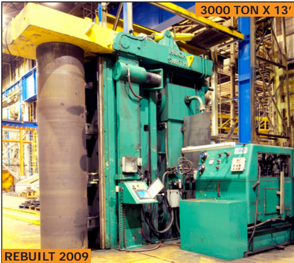
HUGH SMITH vertical plate bending roll (Located in Lester, PA)
