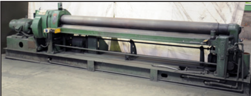
WEBB R3L initial pinch power bending rolls
