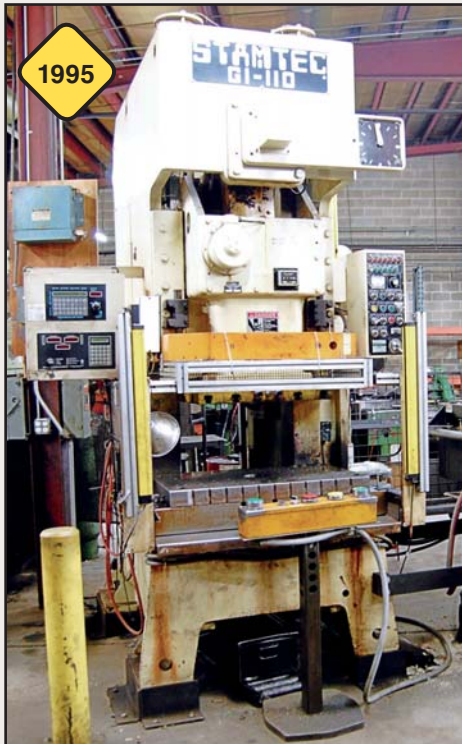
120-Ton Stamtec Mdl. G1-110 Gap Frame Power Press
