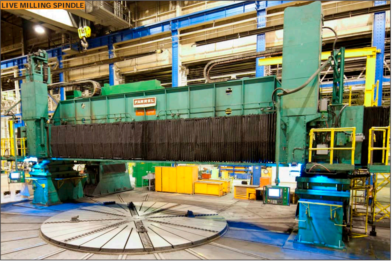
FAREL 313"/ 519" 5-axis CNC vertical boring mill
