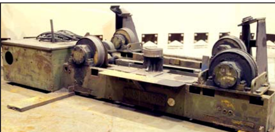
PANDJIRIS 150 ton tank turning rolls
