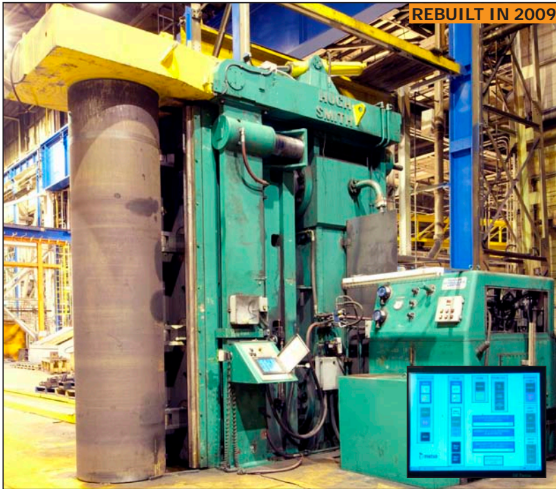
HUGH SMITH 3000 TON x 13' vertical plate bender with PLC control
