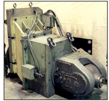
2-axis CNC milling head
