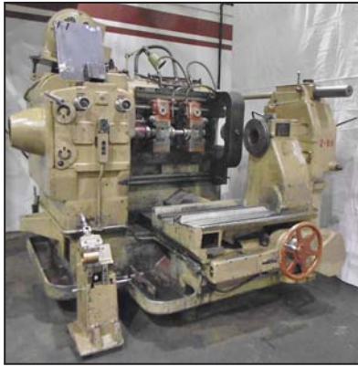
SYKES MODEL 2 gear cutter
