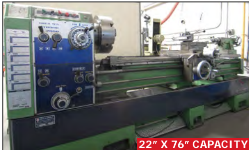
CHIEN YEH STRONG 2000 gap bed engine lathe
