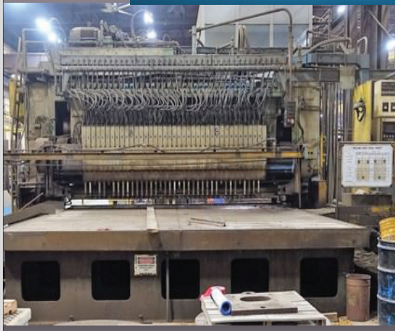
MOLINE 41 SPINDLE CNC TRAVELLING GANTRY MULTI SPINDLE DRILLING MACHINE #27928
